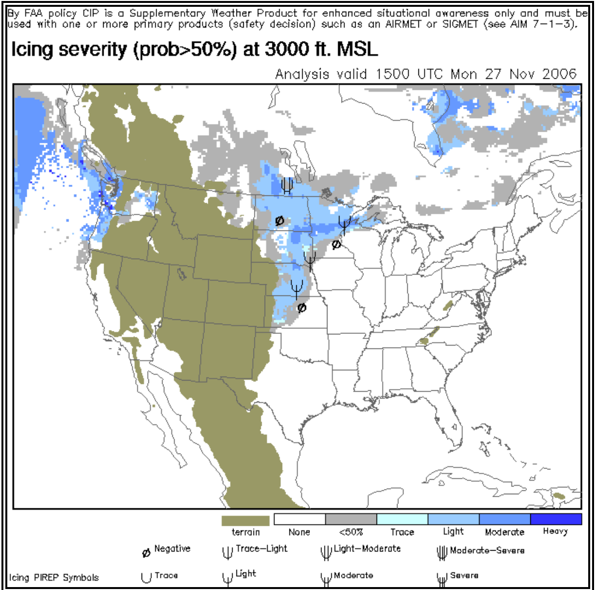
Figure 9-18. CIP Icing Severity Probability > 50% Example
