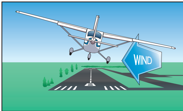
Figure 8-16. Sideslip approach.
