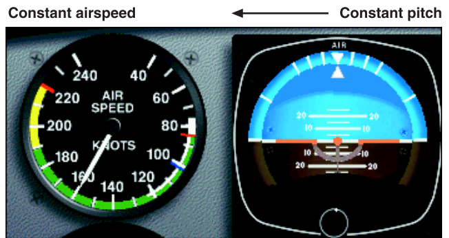
Figure 5-13. Constant power plus constant pitch equals constant airspeed.
