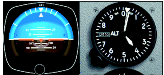
Figure 5-10. Pitch correction, less than 100 feet—1/2 bar low to correct altitude error.
