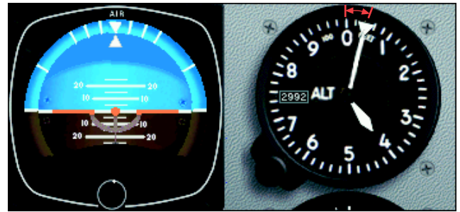
Figure 5-9. Altitude error, less than 100 feet.
